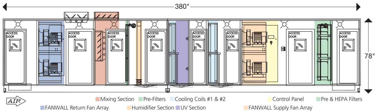
Elevation view of a Temtrol ITF air handler delivering 12,000 cfm @ 5.6" TSP using a FANWALL array for both return and supply fans.
